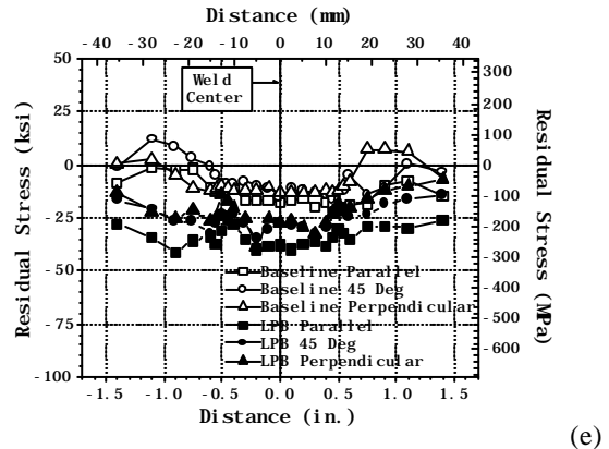
Figure 4: Residual stress measurements in FSW 2219 T8751 aluminum with and without low plasticity burnishing, (a) weld surface, (b) 1/4 thickness, (c) 1/2 thickness, (d) 3/4 thickness, and (e) weld root surface.
