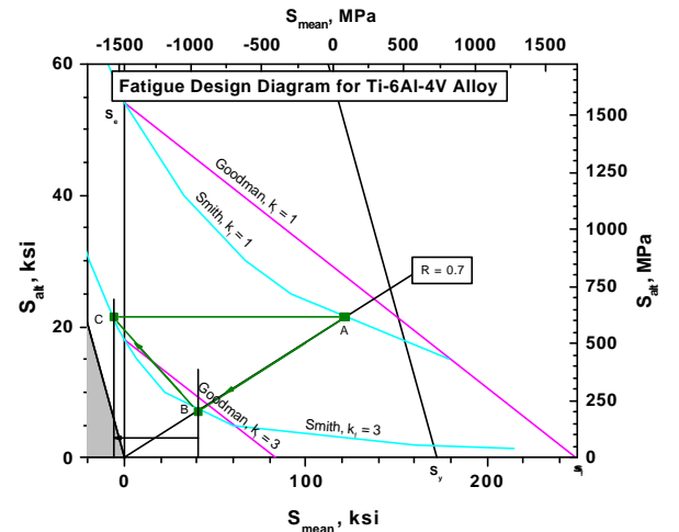
FIG 19. Section of the Fatigue Design Diagram illustrating the required magnitude of compression to fully mitigate the effect of FOD of k_t of 3.
