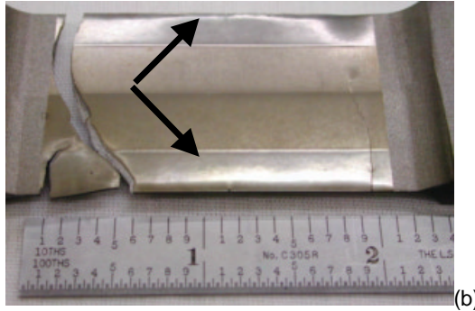
FIG. 10. (a) Optical fractograph of a SEB feature specimen with LPB treatment showing crack initiation from sub surface regions (arrow), LPB + 0.5 mm (0.020 in) FOD, R=0.1 , \sigma_{max}=690 MPa (100 ksi), N_f = 800,038 cycles, (b) Failure of a DEB feature specimen with LPB treatment showing initiation in a remote area in spite of the presence of 0.5 mm (0.020 in.) FOD (arrows) on both edges of the specimen. R=-1 , \sigma_{max} = 480 MPa (70 ksi), N_f = 174,315 cycles.
