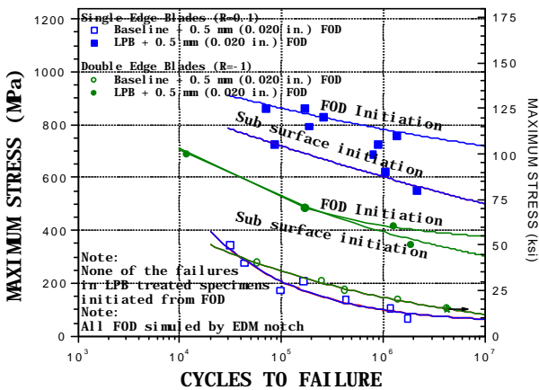
FIG. 9. HCF test results for the blade edge simulation feature specimens.
