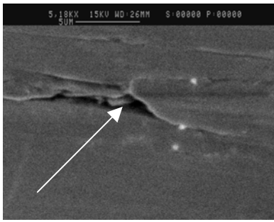
Figure 9e: Cracking on the gage surface just below crack initiation site at the initial stage of formation of a corrosion pit (arrow).
