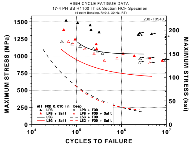
Figure 5. Corrosion fatigue and HCF results for LPB treatment. Baseline data for LSG treatment (fitted lines from Figure 3) are shown for comparison.
