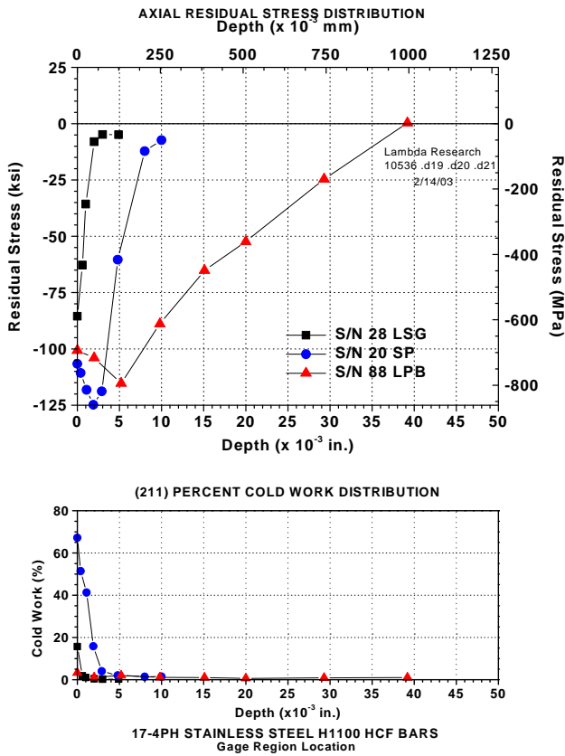
Figure 2. Residual stress distribution for LSG, SP and LPB processed (and fatigue tested, all in air) specimens. S/N28 (LSG): S_{max} = 140 ksi (~965 MPa); N_f = 3,303,607 cycles, S/N20 (SP): S_{max} = 185 ksi (~1275 MPa); N_f = 148,980 cycles, S/N88 (LPB): S_{max} = 210 ksi (~1,450 MPa); N_f = 200,445 cycles
