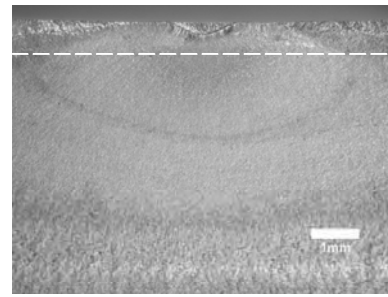
Figure 10a: Optical fractograph of corrosion fatigue tested notched (0.010 in.) specimen LPB + salt 0.010 in. EDM notch. S_{max} = 140 ksi (965 MPa); N_f = 794,917 cycles – note the notch depth is smaller than the approximate LPB processed zone (dotted white line).
