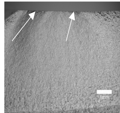
Figure 7a: LSG, Smax = 170 ksi (1,170 MPa), Nf = 103,997 cycles – arrows indicate multiple crack initiation sites.
