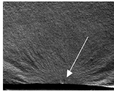
Figure 9a: LPB + salt unnotched, S_{max} = 150 ksi (1,035 MPa), N_f = 316,613 cycles – arrow indicates initiation
