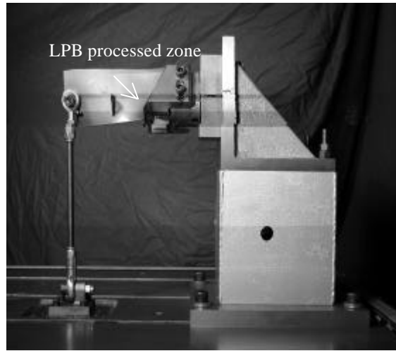
Figure 8 - Photograph showing the cantilever-loading fixture for fatigue testing of the first stage fan blade. Note the LPB patch along the (upper) leading edge of the blade.
