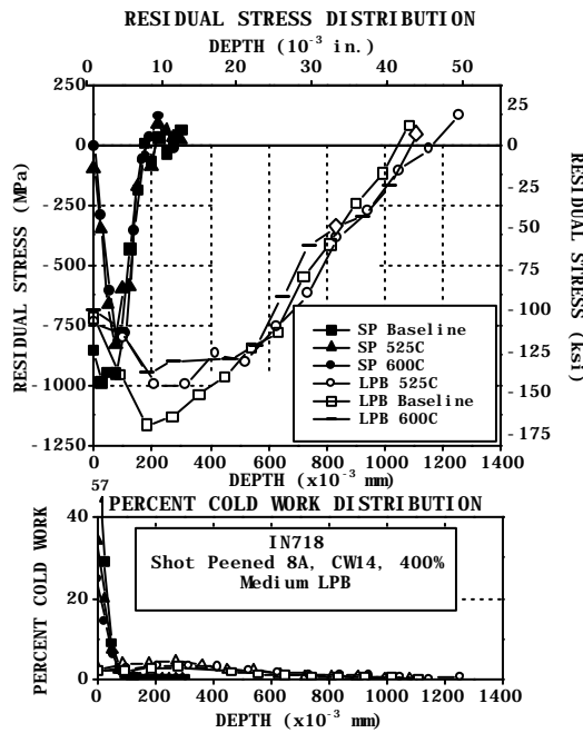
Figure 3 – Residual Stress and cold work depth profiles for IN718 before and after exposure to service temperature of 525° and 600°C for 100 hrs.
