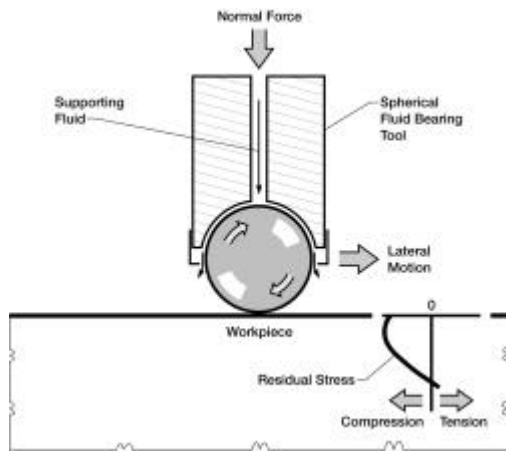
Figure 1- LPB Schematic
