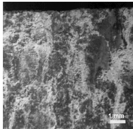
Figure 4 - Macroscopic appearance of a specimen after 100-hr. exposure showing patches of Al 2 O 3 corrosion product.
