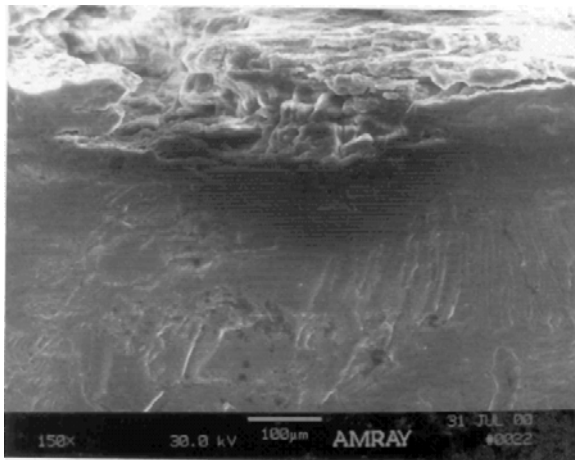
Figure 5B - Microscopic appearance of the fatigue origin at the site of corrosion pit shown in 5A after 100 hr. salt for exposure.
