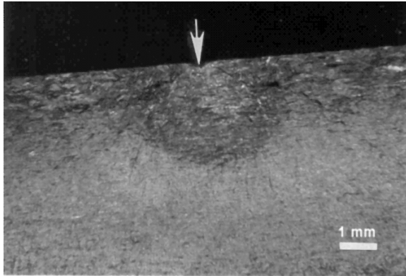
Figure 5A- Arrow indicates macroscopic appearance of fatigue origin at the site of corrosion after 100 hr. salt fog exposure.
