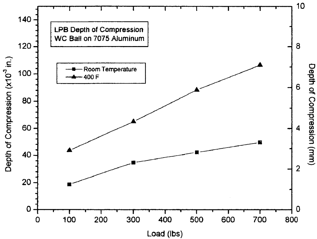
Depth of compression achieved with increasing load in spherical ball burnishing using a 0.75 in. ball at room and elevated temperature of 400° F.
