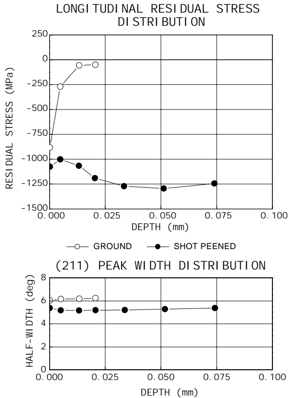
Fig. 8 Residual Stress and Peak Width Distributions Produced by Shot Peening (18A) and Grinding of Carburized 8620 Steel.
