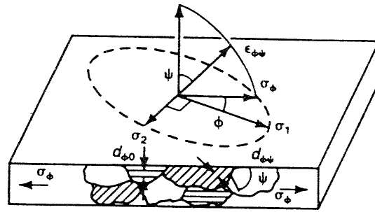
Fig. 1 Plane Stress at a Free Surface
